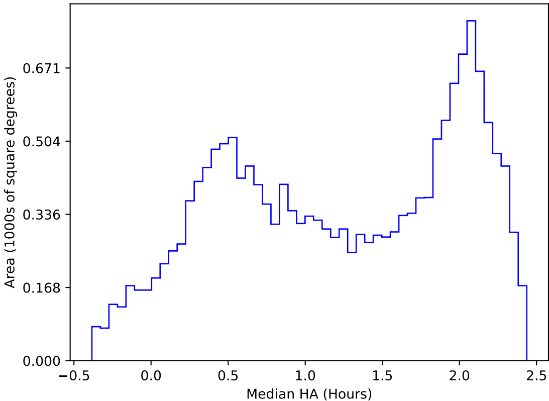
internal_u_expt38_nscale1.1v3.4_10yrs WFD y band: Median HA
