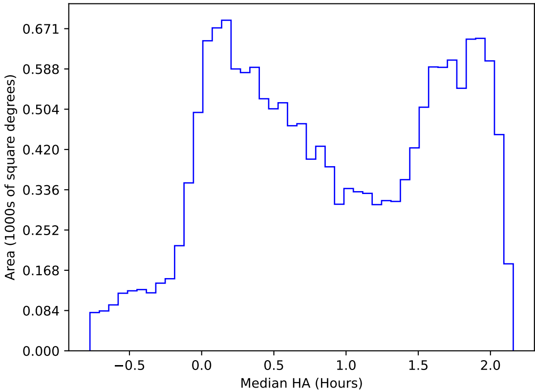
internal_u_expt38_nscale1.1v3.4_10yrs WFD r band: Median HA
