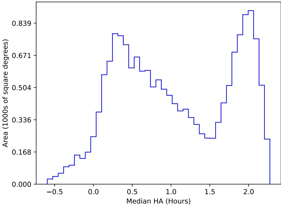
internal_u_expt38_nscale1.1v3.4_10yrs WFD i band: Median HA
