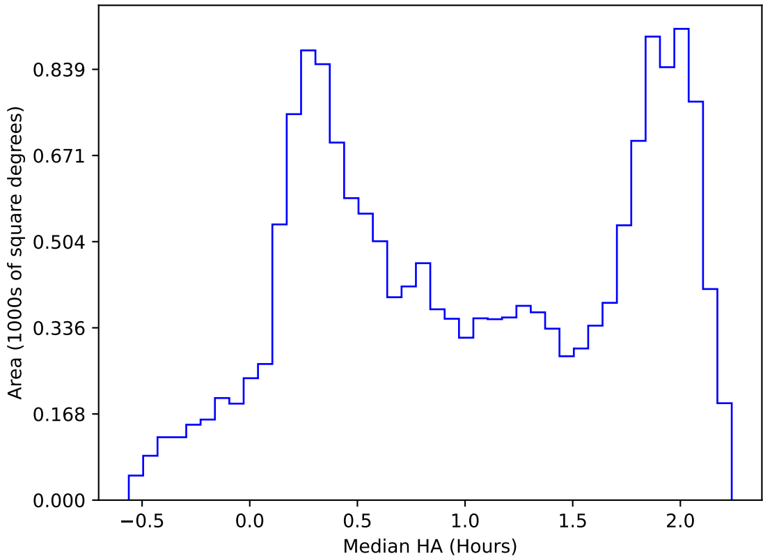
internal_u_expt38_nscale1.1v3.4_10yrs WFD all bands: Median HA
