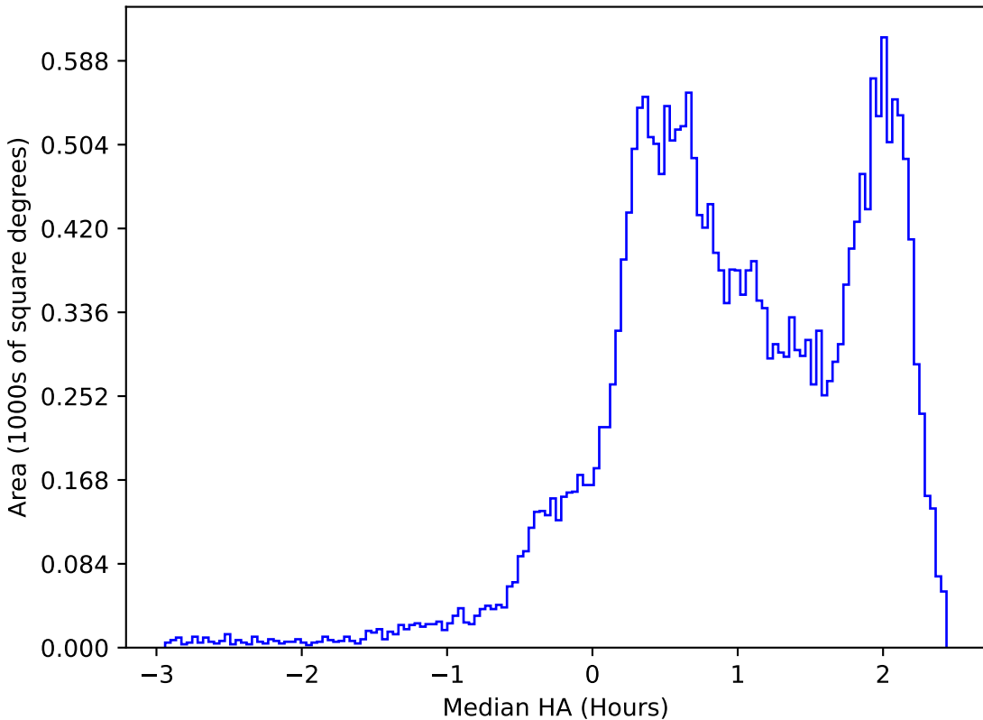
internal_u_expt38_nscale1.1v3.4_10yrs All sky z band: Median HA
