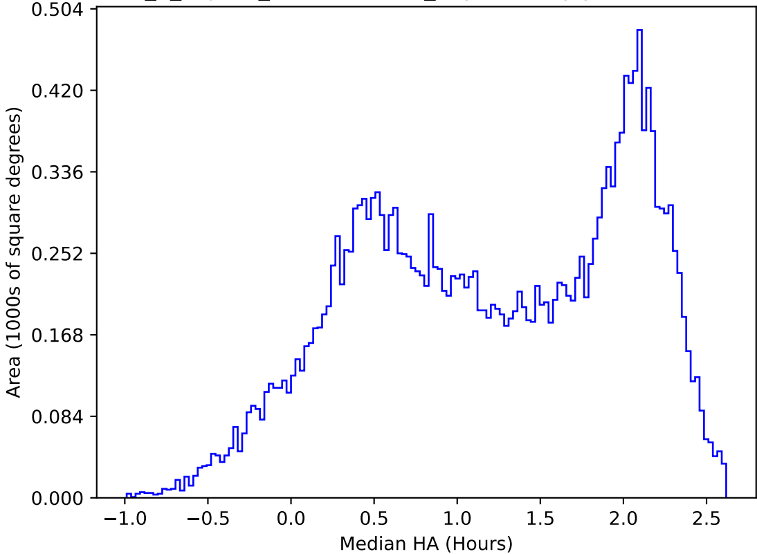
internal_u_expt38_nscale1.1v3.4_10yrs All sky y band: Median HA
