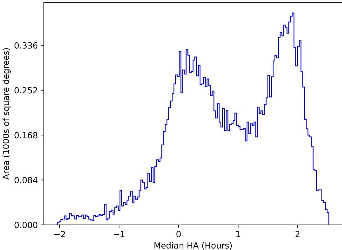
internal_u_expt38_nscale1.1v3.4_10yrs All sky u band: Median HA
