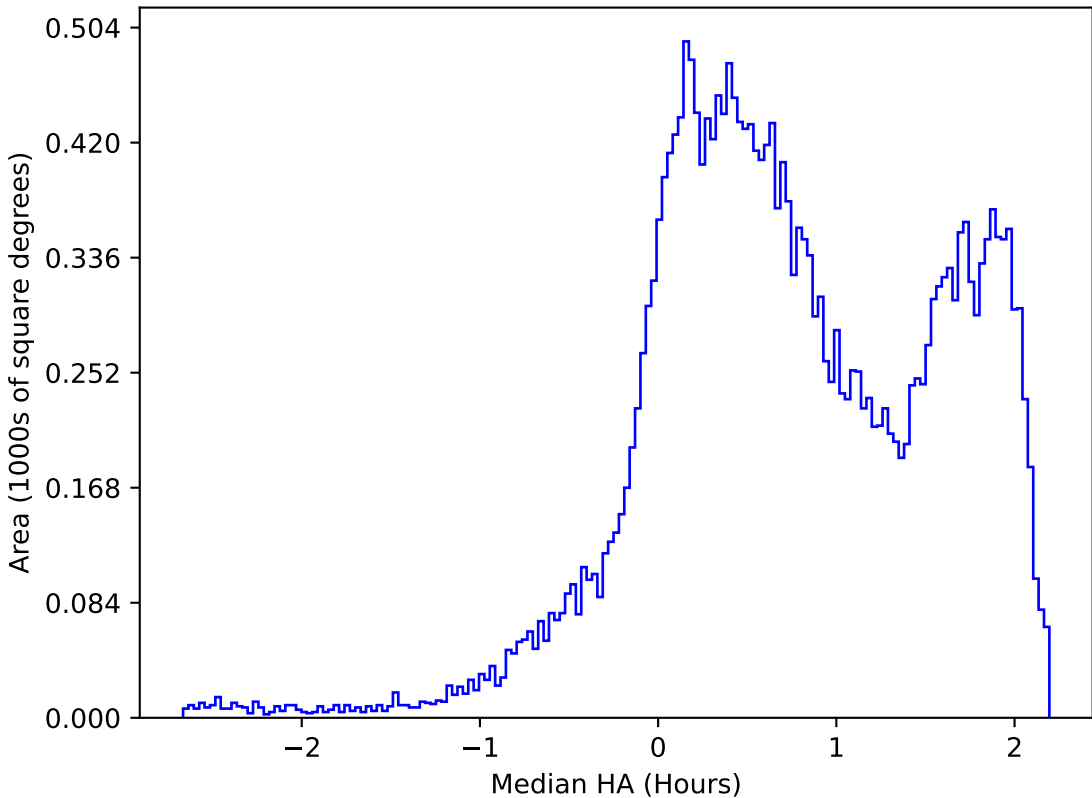
internal_u_expt38_nscale1.1v3.4_10yrs All sky r band: Median HA
