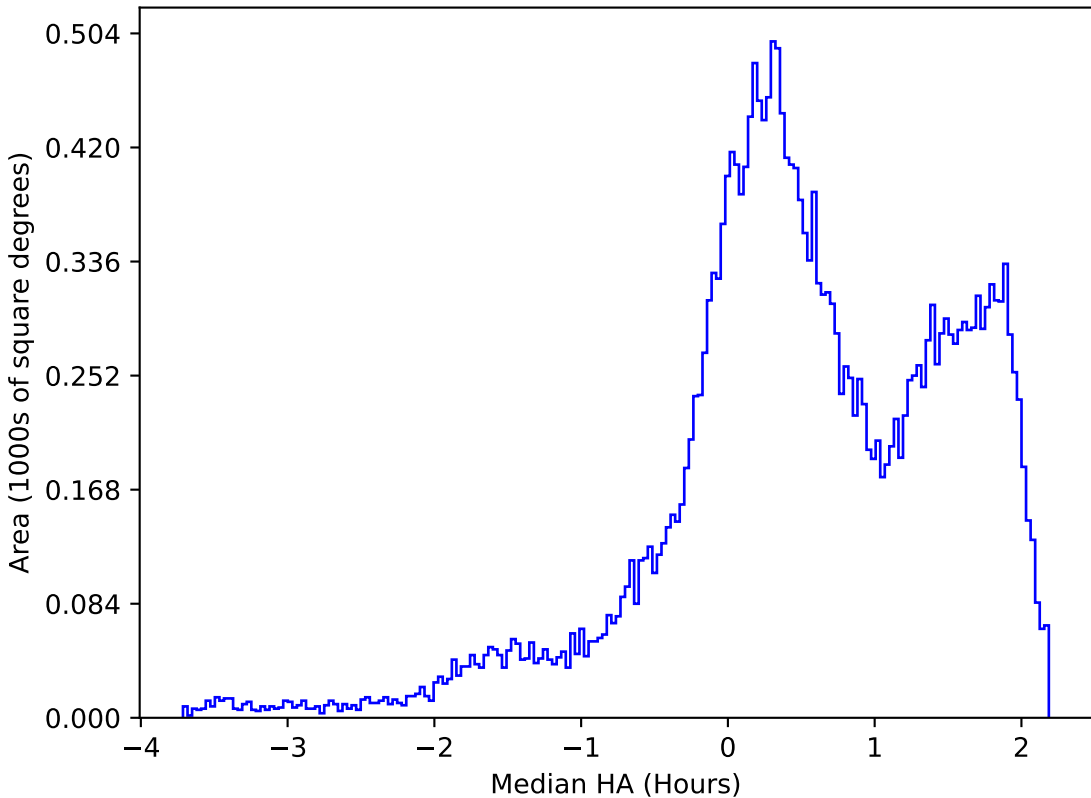
internal_u_expt38_nscale1.1v3.4_10yrs All sky g band: Median HA
