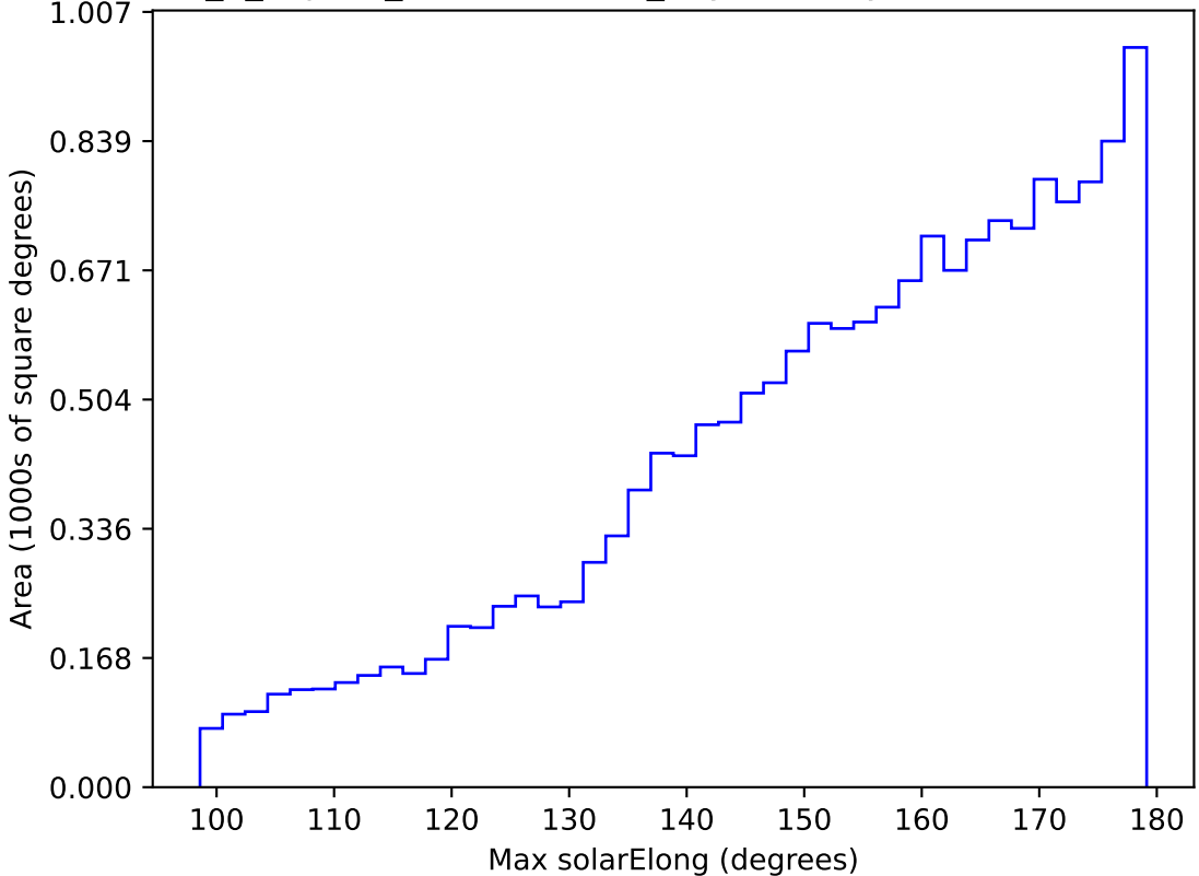
internal_u_expt38_nscale1.1v3.4_10yrs WFD y band: Max solarElong
