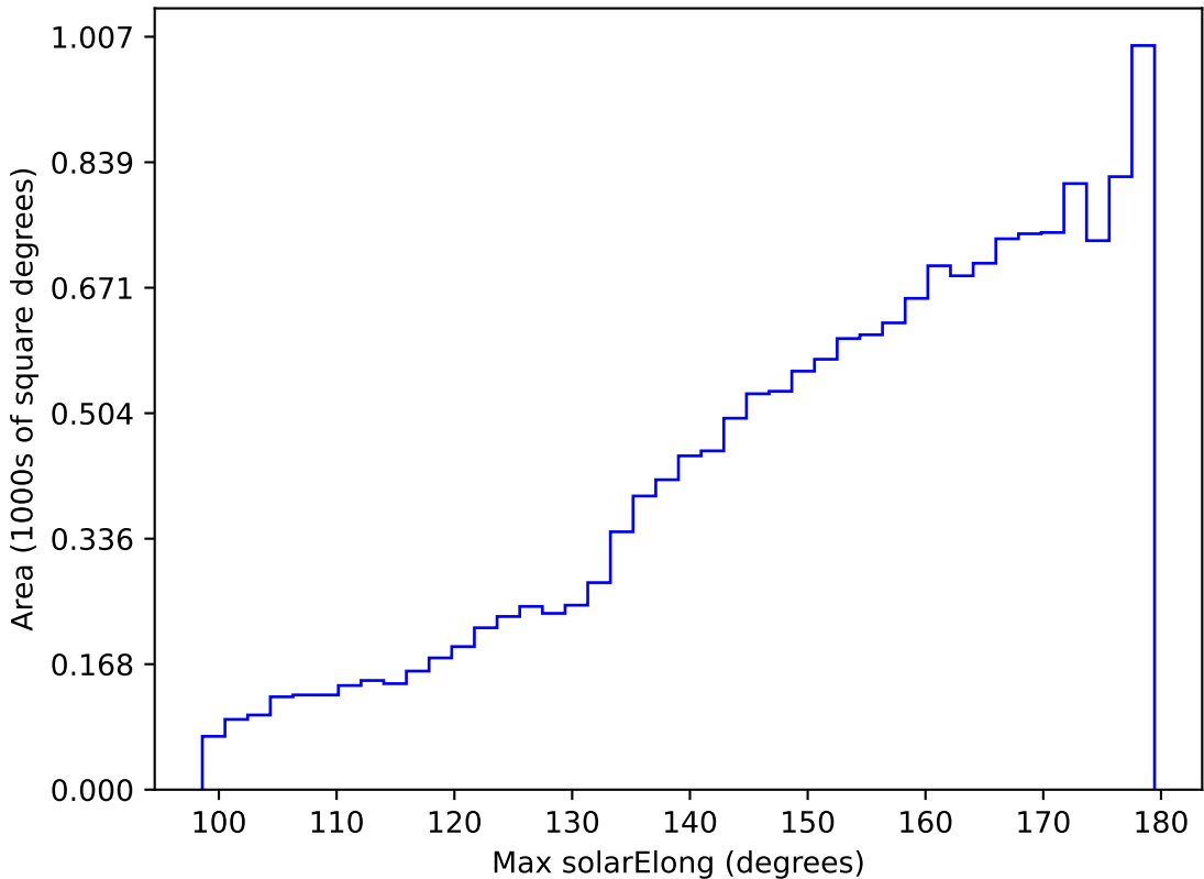
internal_u_expt38_nscale1.1v3.4_10yrs WFD r band: Max solarElong
