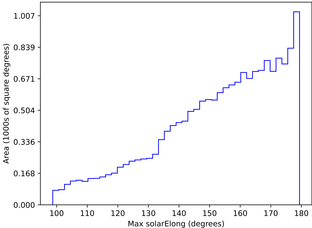
internal_u_expt38_nscale1.1v3.4_10yrs WFD i band: Max solarElong
