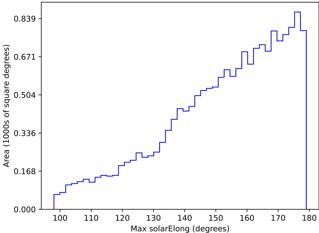
internal_u_expt38_nscale1.1v3.4_10yrs WFD g band: Max solarElong
