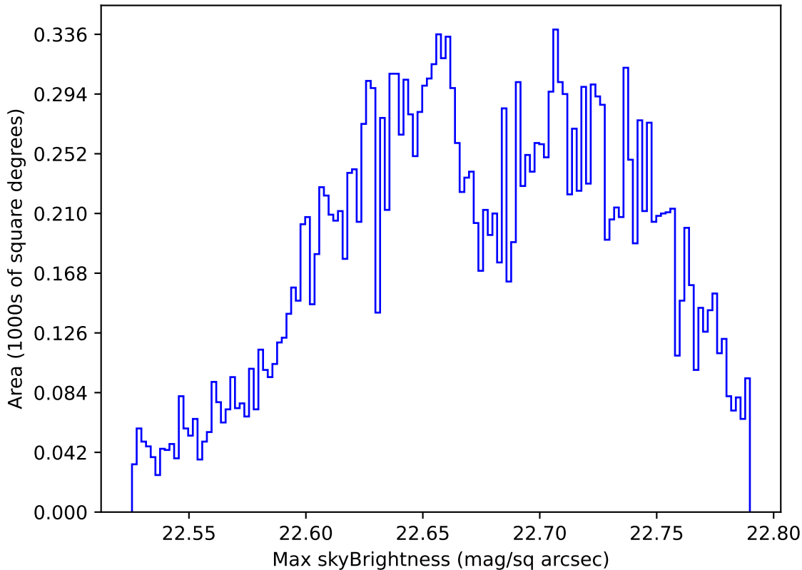
internal_u_expt38_nscale1.1v3.4_10yrs Yr 1 u band: Max skyBrightness
