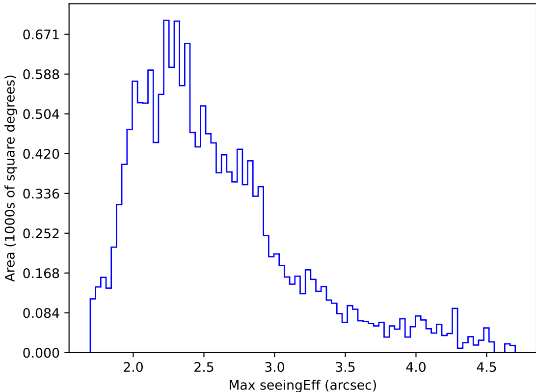
internal_u_expt38_nscale1.1v3.4_10yrs WFD z band: Max seeingEff
