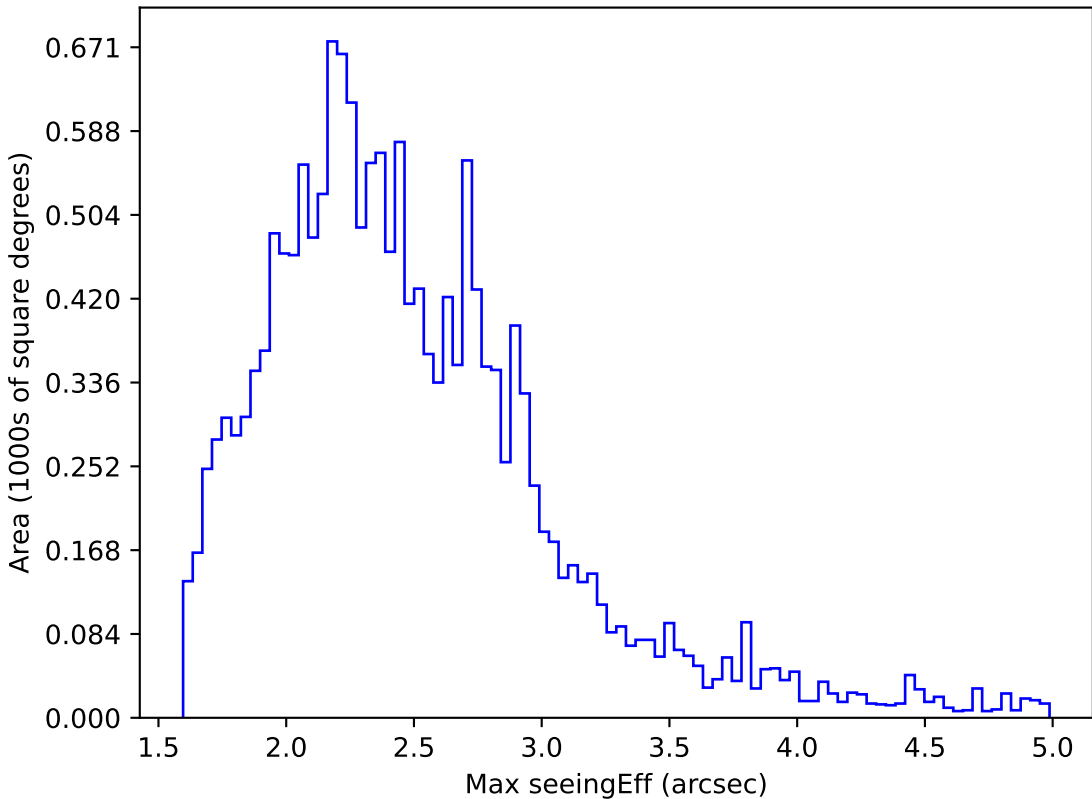
internal_u_expt38_nscale1.1v3.4_10yrs WFD y band: Max seeingEff
