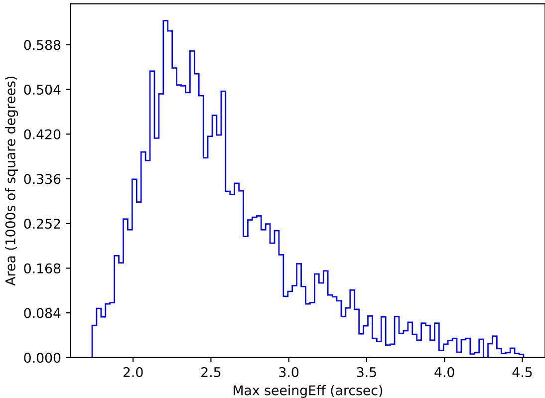
internal_u_expt38_nscale1.1v3.4_10yrs WFD u band: Max seeingEff
