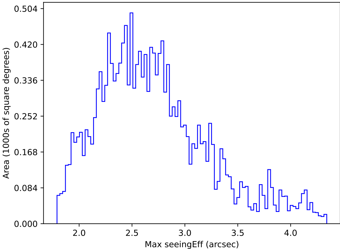
internal_u_expt38_nscale1.1v3.4_10yrs WFD r band: Max seeingEff
