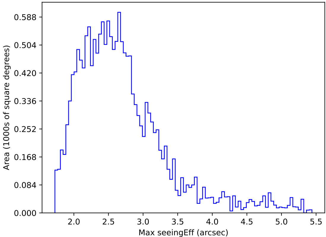
internal_u_expt38_nscale1.1v3.4_10yrs WFD i band: Max seeingEff
