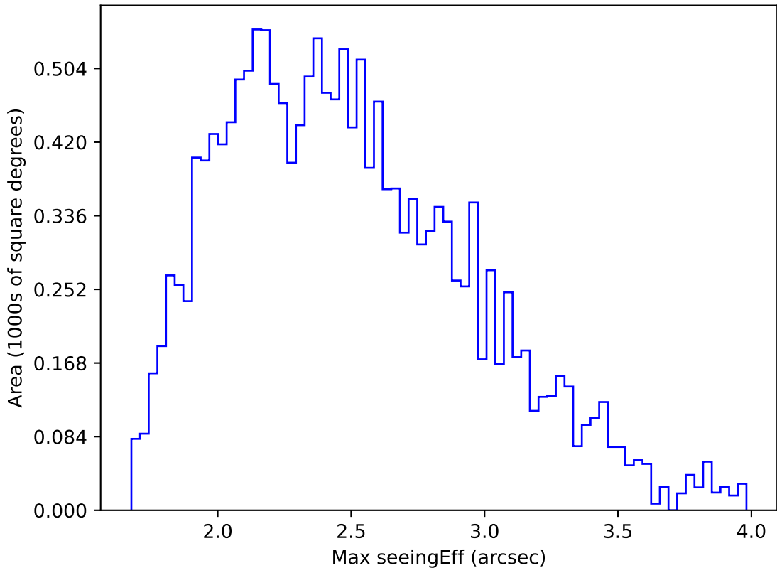
internal_u_expt38_nscale1.1v3.4_10yrs WFD g band: Max seeingEff
