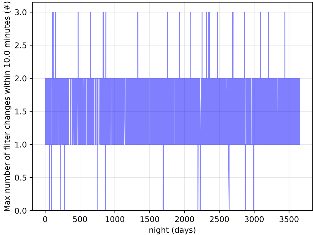
internal_u_expt38_nscale1.1v3.4_10yrs Per Night: Max number of filter changes within 10.0 minutes
