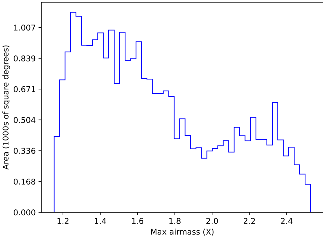
internal_u_expt38_nscale1.1v3.4_10yrs Yr 1 r band: Max airmass
