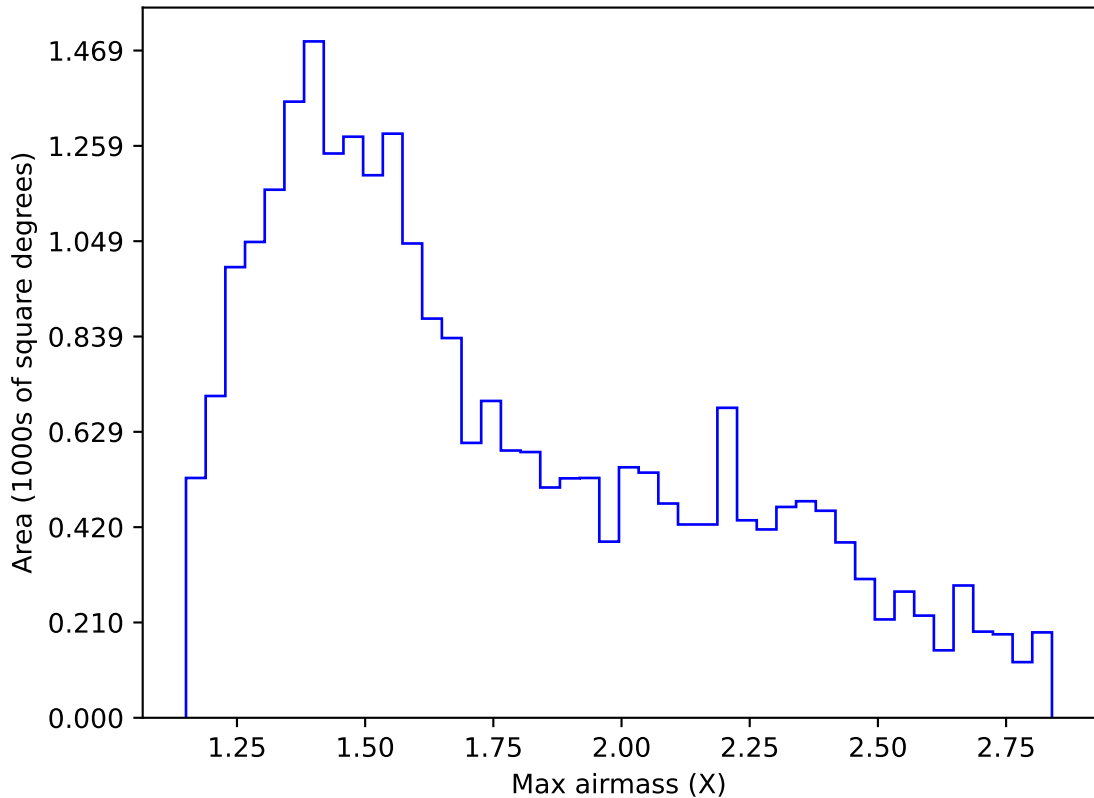
internal_u_expt38_nscale1.1v3.4_10yrs Yr 1 i band: Max airmass
