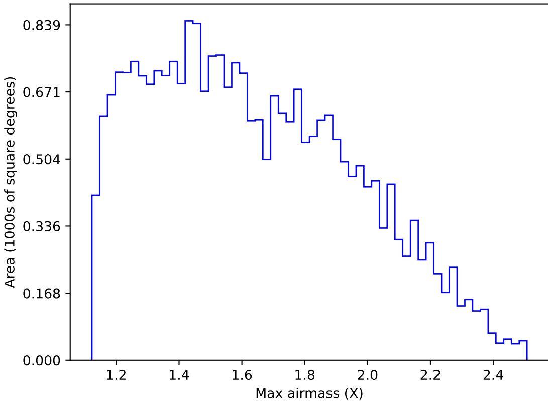
internal_u_expt38_nscale1.1v3.4_10yrs Yr 1 g band: Max airmass
