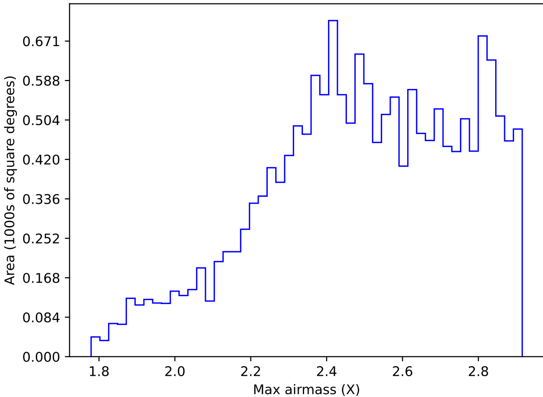
internal_u_expt38_nscale1.1v3.4_10yrs WFD z band: Max airmass
