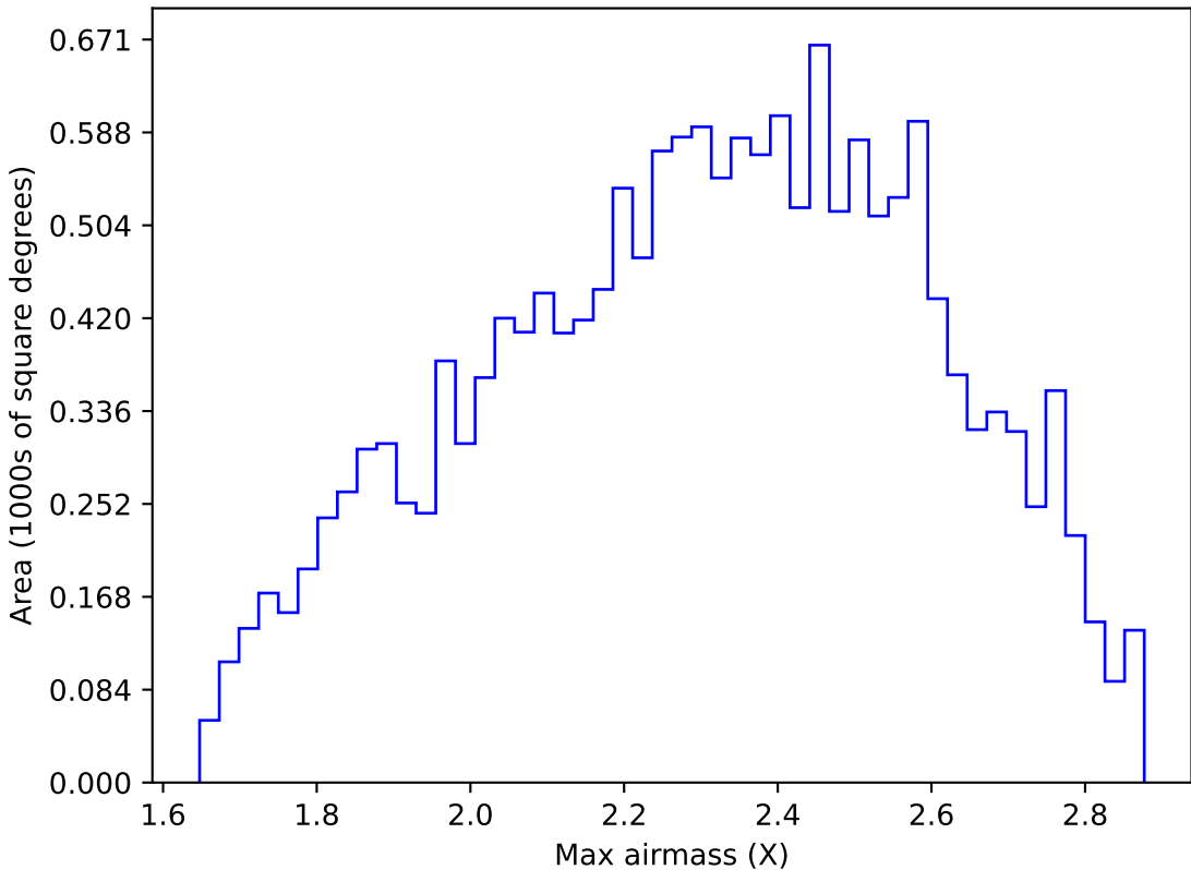
internal_u_expt38_nscale1.1v3.4_10yrs WFD y band: Max airmass
