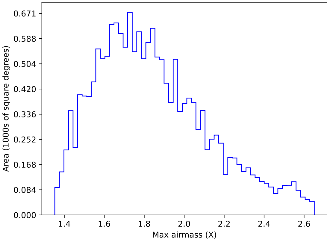
internal_u_expt38_nscale1.1v3.4_10yrs WFD u band: Max airmass
