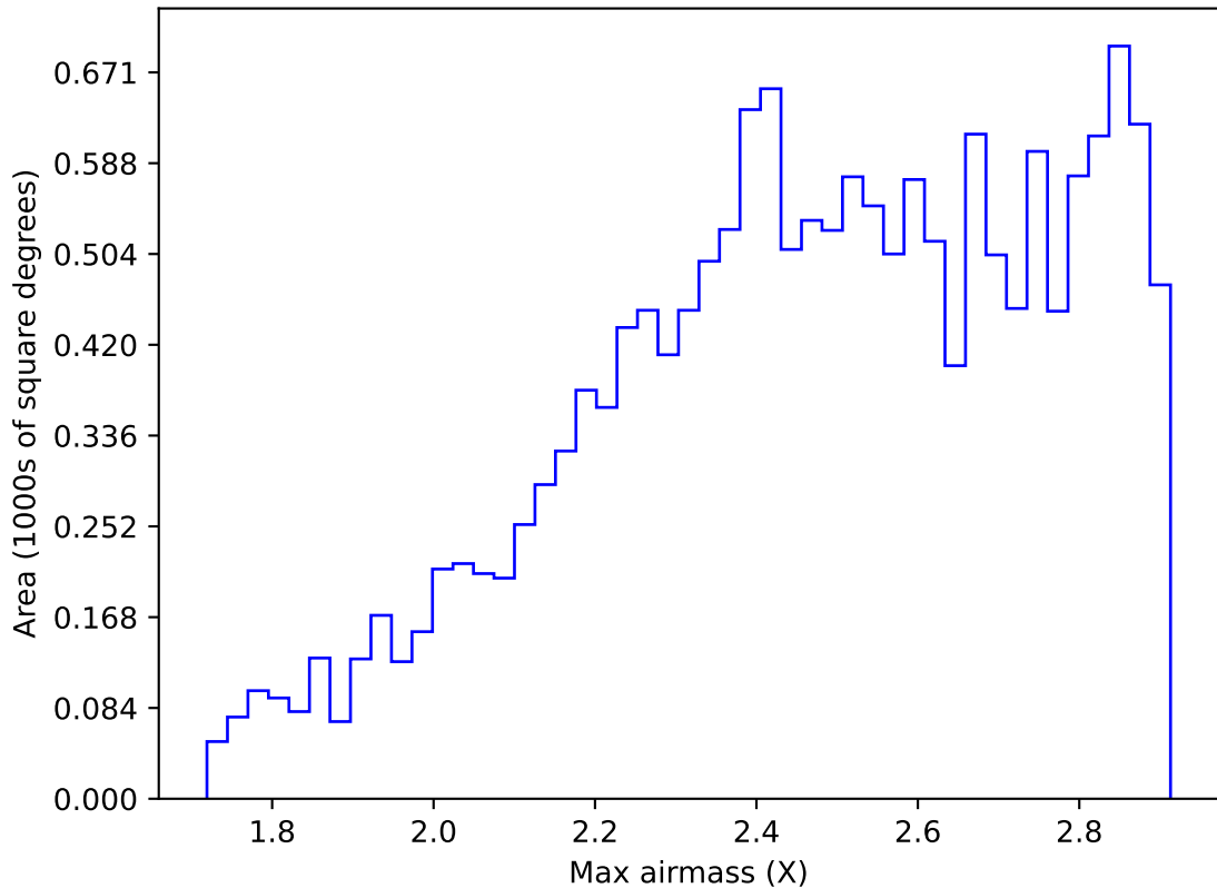
internal_u_expt38_nscale1.1v3.4_10yrs WFD i band: Max airmass
