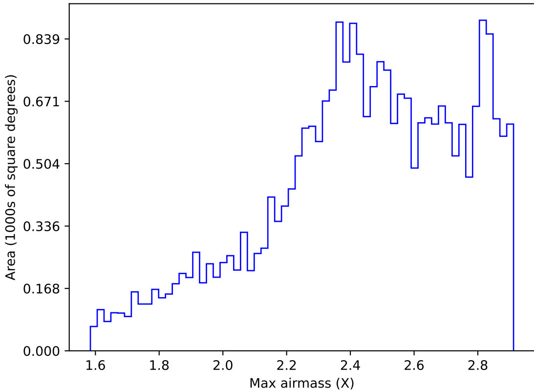
internal_u_expt38_nscale1.1v3.4_10yrs All sky z band: Max airmass
