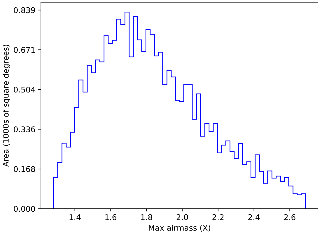
internal_u_expt38_nscale1.1v3.4_10yrs All sky u band: Max airmass
