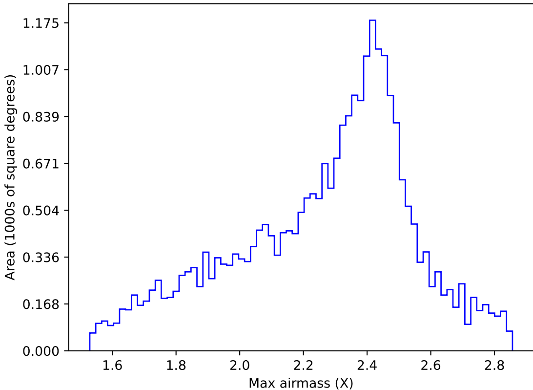
internal_u_expt38_nscale1.1v3.4_10yrs All sky r band: Max airmass
