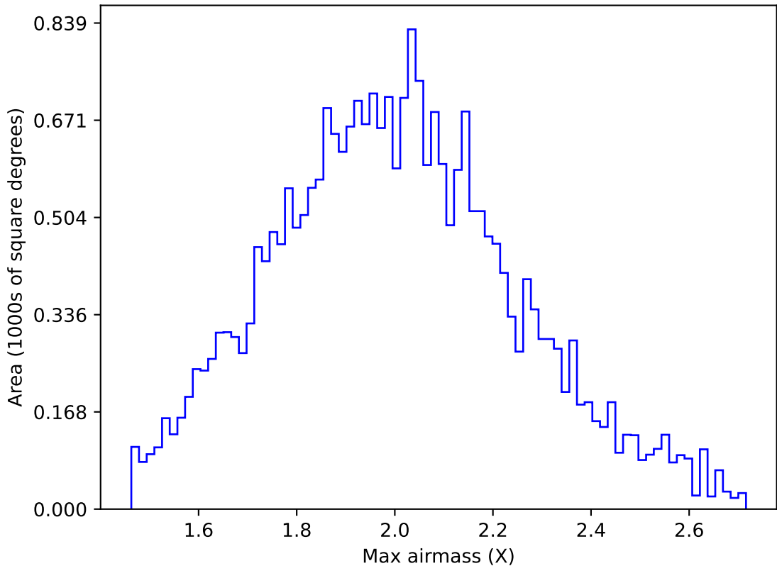
internal_u_expt38_nscale1.1v3.4_10yrs All sky g band: Max airmass
