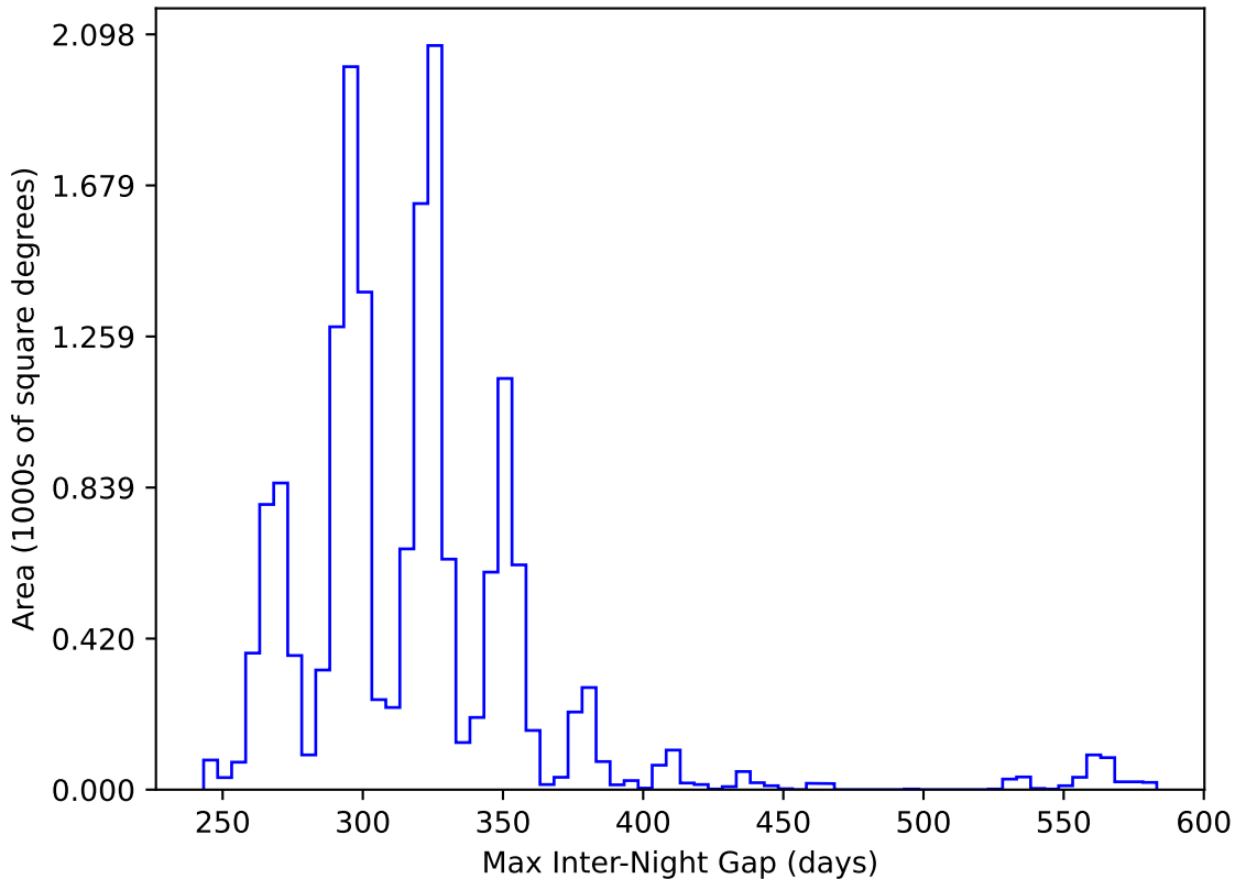
internal_u_expt38_nscale1.1v3.4_10yrs WFD y band: Max Inter-Night Gap
