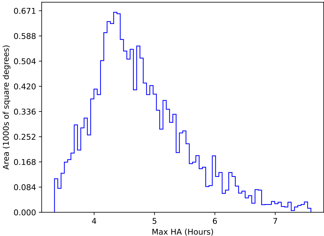
internal_u_expt38_nscale1.1v3.4_10yrs WFD y band: Max HA
