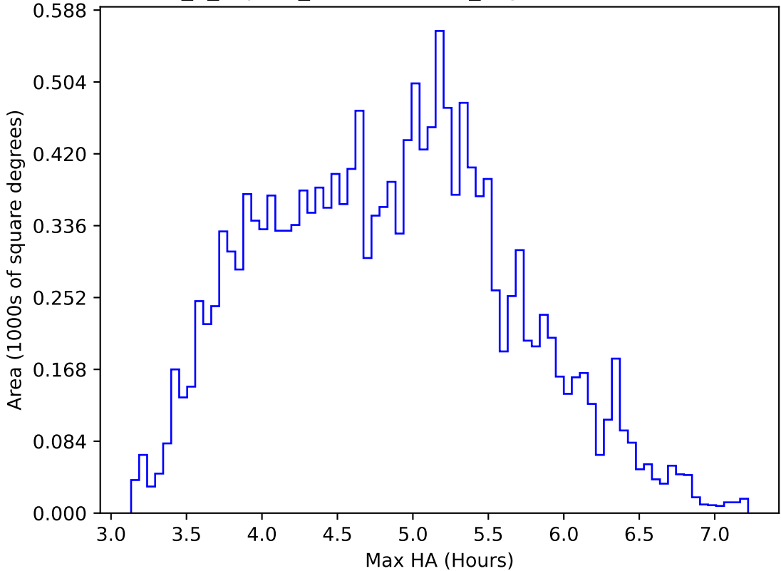
internal_u_expt38_nscale1.1v3.4_10yrs WFD i band: Max HA
