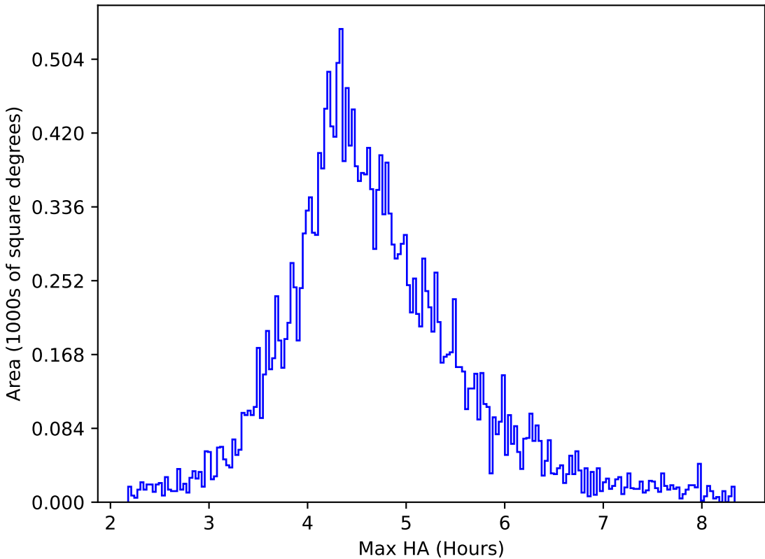
internal_u_expt38_nscale1.1v3.4_10yrs All sky y band: Max HA
