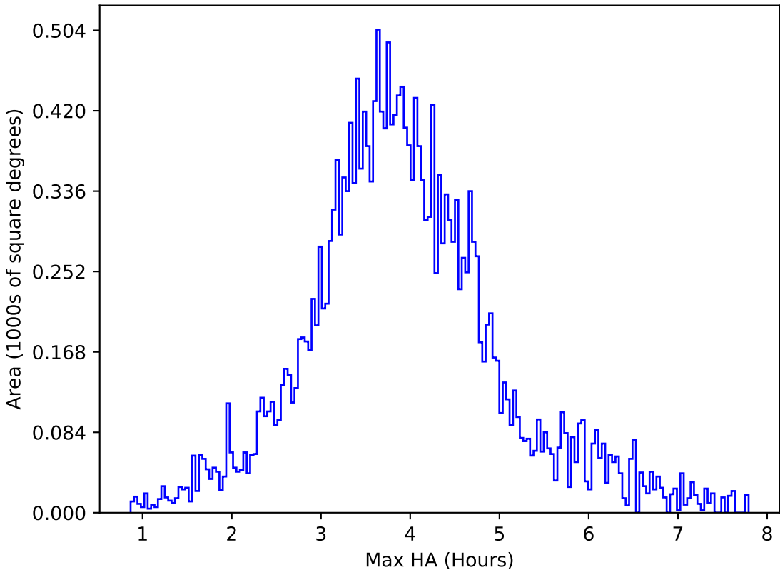
internal_u_expt38_nscale1.1v3.4_10yrs All sky u band: Max HA
