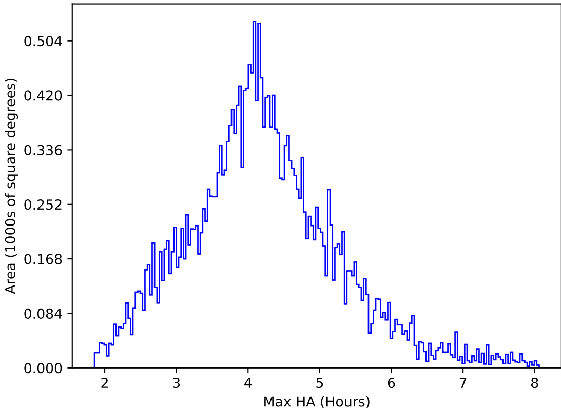
internal_u_expt38_nscale1.1v3.4_10yrs All sky r band: Max HA
