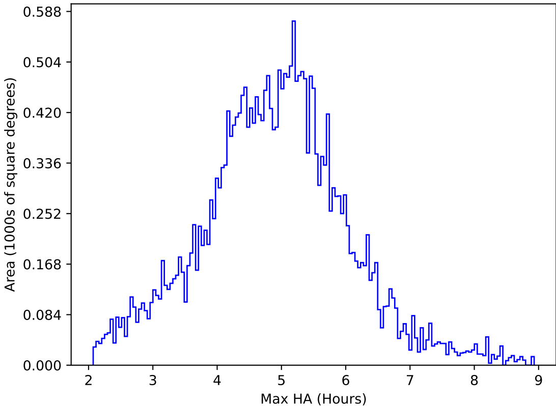
internal_u_expt38_nscale1.1v3.4_10yrs All sky all bands: Max HA
