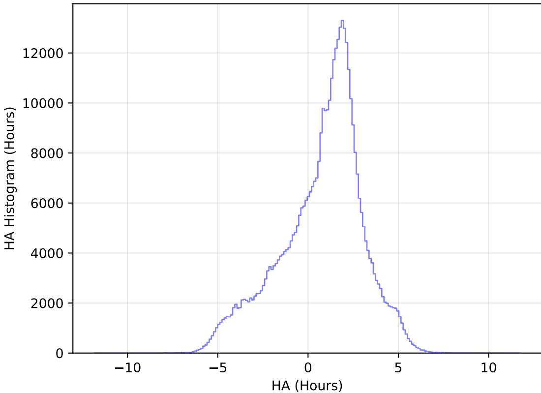
internal_u_expt38_nscale1.1v3.4_10yrs WFD z band: HA Histogram
