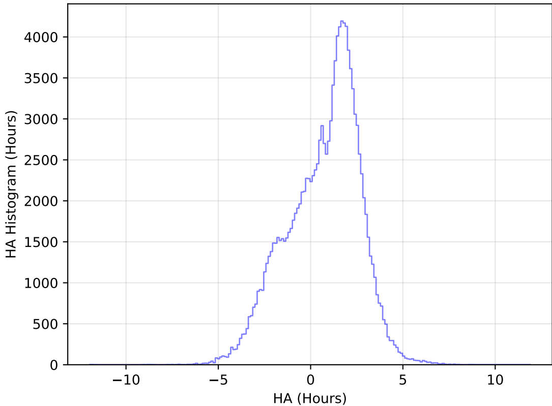
internal_u_expt38_nscale1.1v3.4_10yrs WFD u band: HA Histogram
