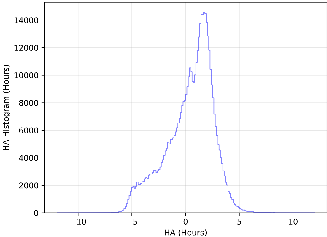
internal_u_expt38_nscale1.1v3.4_10yrs WFD r band: HA Histogram
