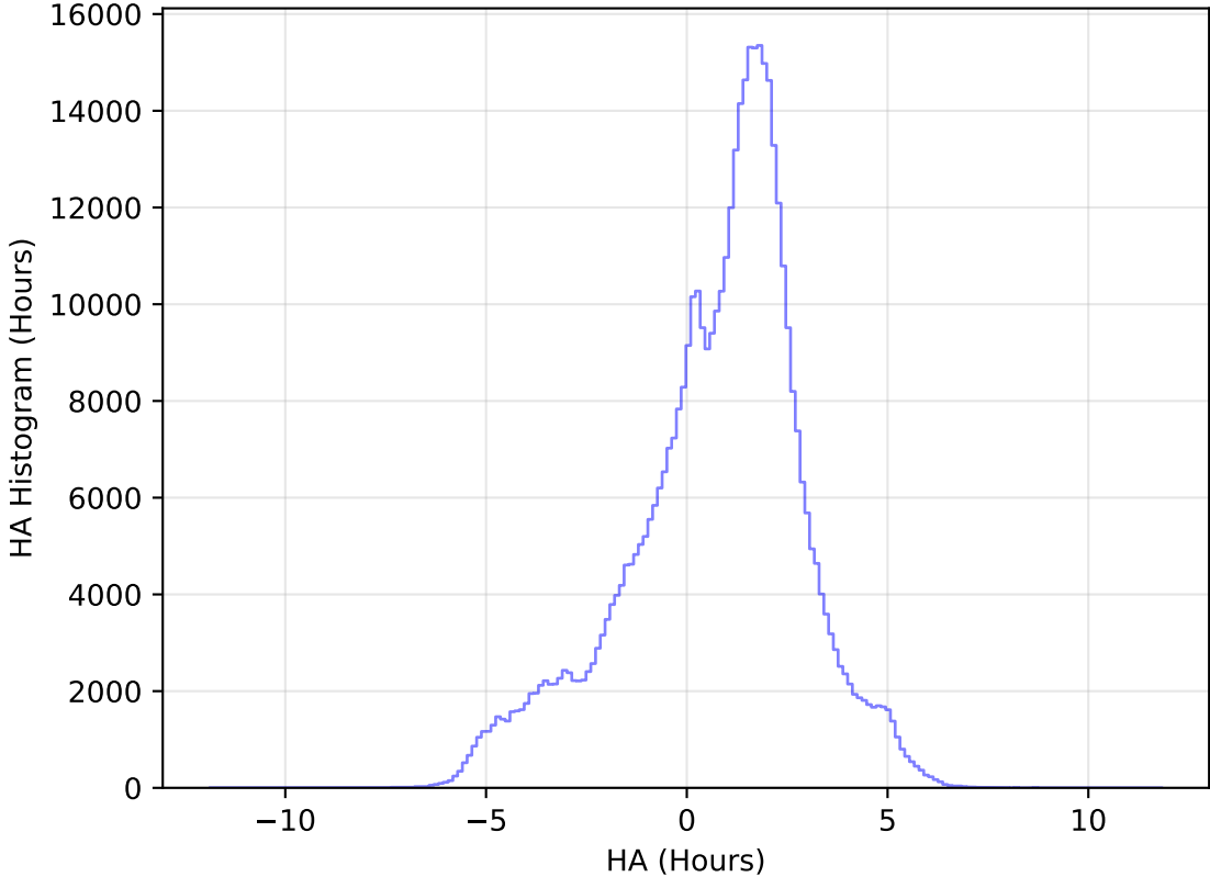
internal_u_expt38_nscale1.1v3.4_10yrs WFD i band: HA Histogram
