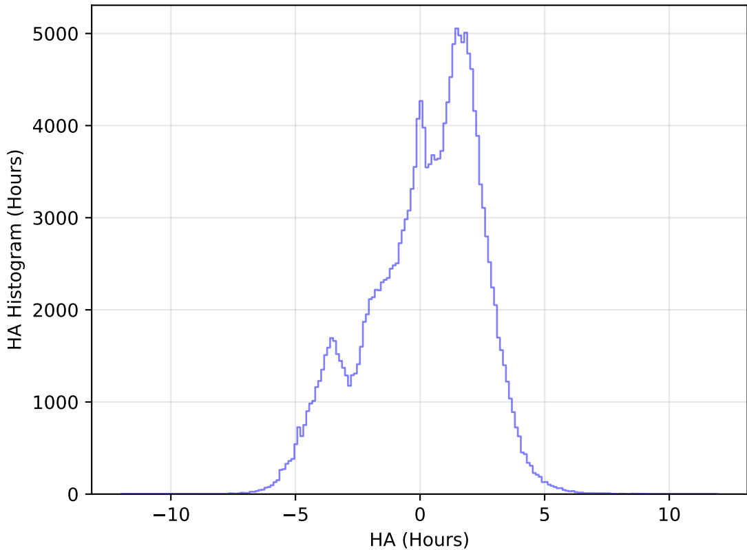
internal_u_expt38_nscale1.1v3.4_10yrs WFD g band: HA Histogram
