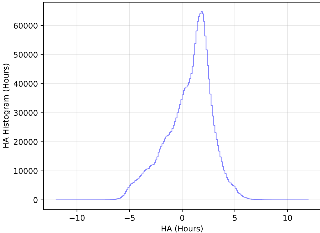
internal_u_expt38_nscale1.1v3.4_10yrs WFD all bands: HA Histogram
