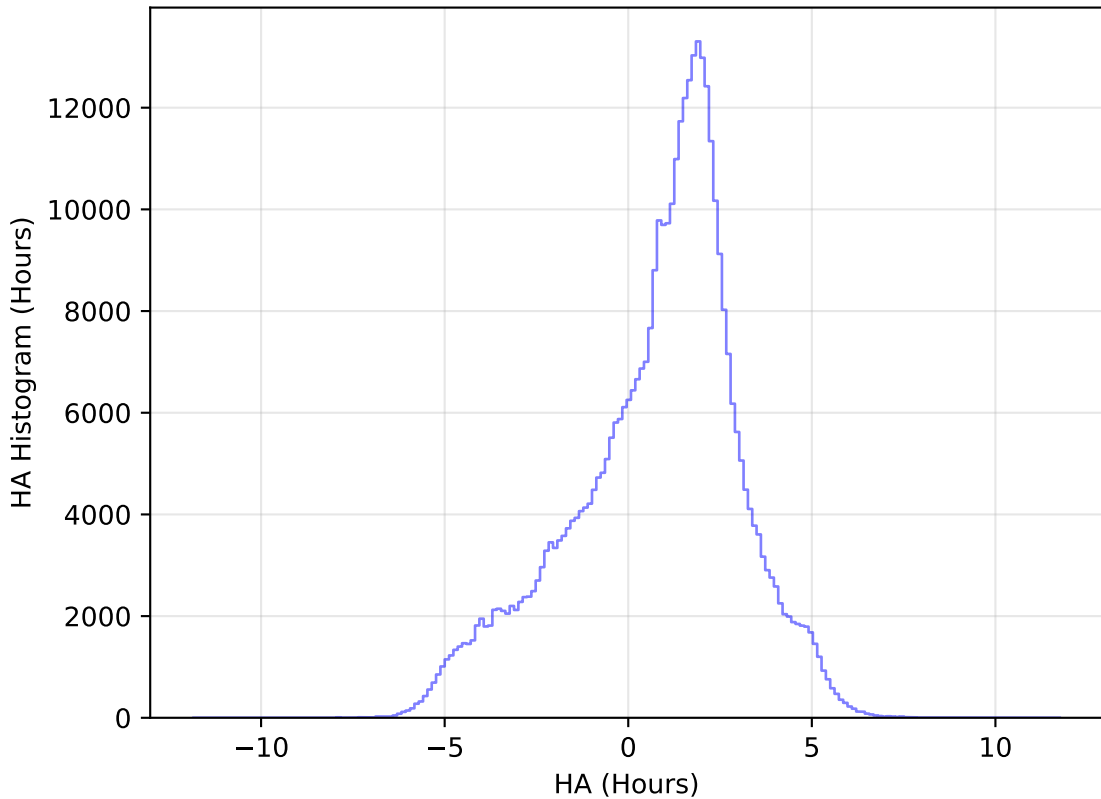
internal_u_expt38_nscale1.1v3.4_10yrs All sky z band: HA Histogram
