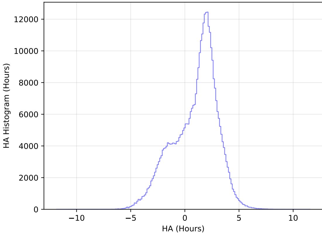
internal_u_expt38_nscale1.1v3.4_10yrs All sky y band: HA Histogram
