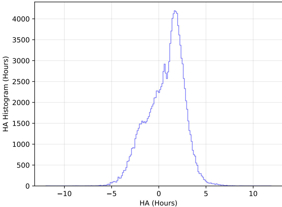
internal_u_expt38_nscale1.1v3.4_10yrs All sky u band: HA Histogram
