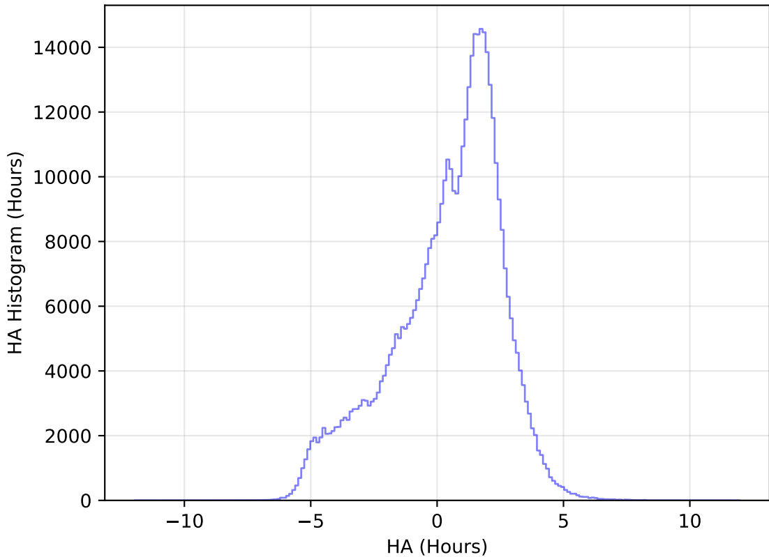
internal_u_expt38_nscale1.1v3.4_10yrs All sky r band: HA Histogram
