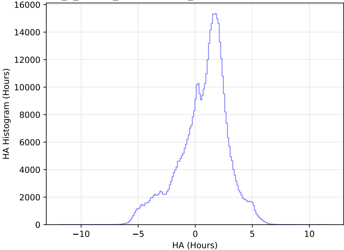
internal_u_expt38_nscale1.1v3.4_10yrs All sky i band: HA Histogram
